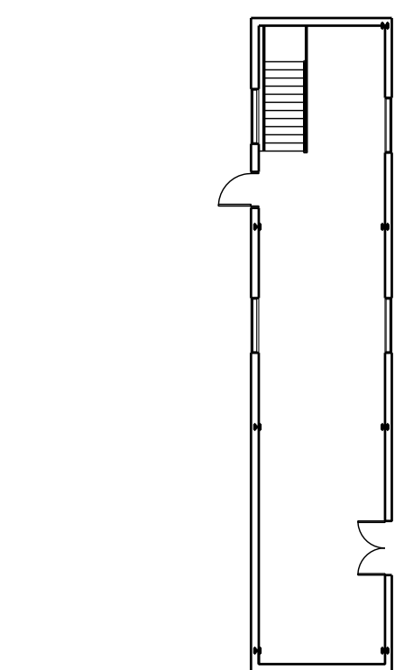
SECOND FLOOR 785 sq. ft. SCALE: 1/16" = 1'-0" NORTH
