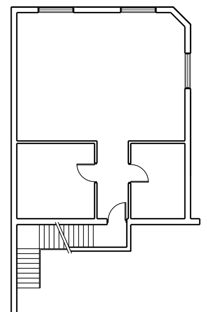
SECOND FLOOR 1,122 sq. ft. SCALE: 1/16" = 1'-0" NORTH
